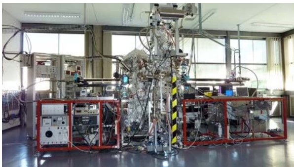
ARPES & XPS
